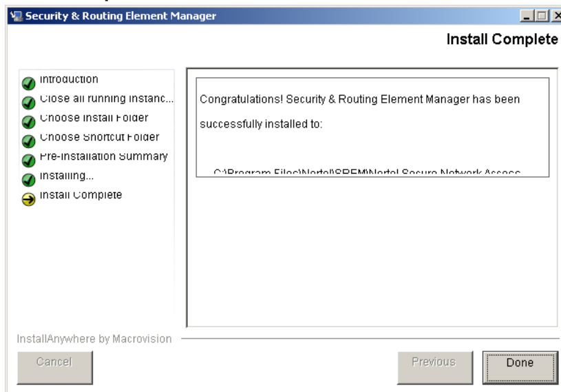
Figure 12 Install Complete
